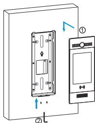
Flush Mounting & Plasterboard mounting
